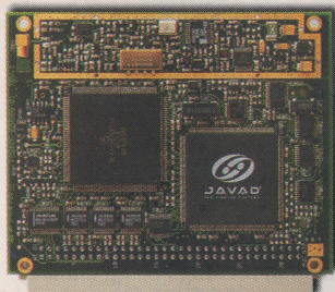
20 channel GPS L1+L2
